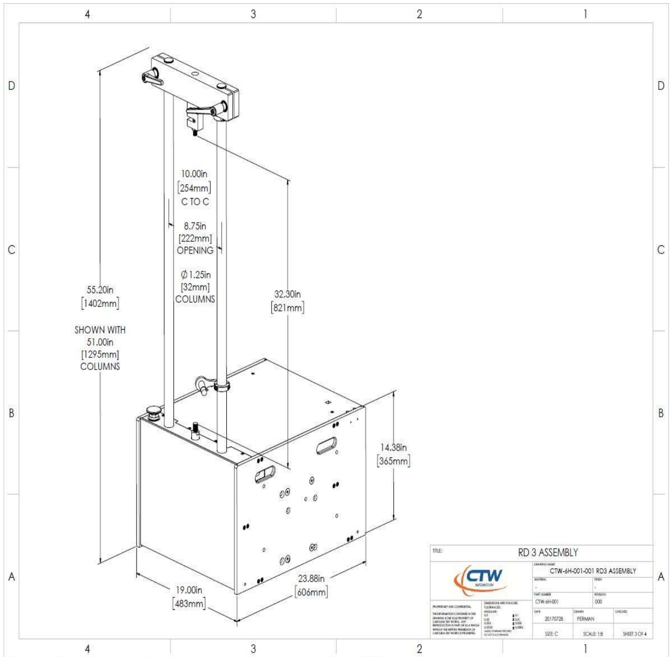
General Dimensional Outline of RD2 and RD3
