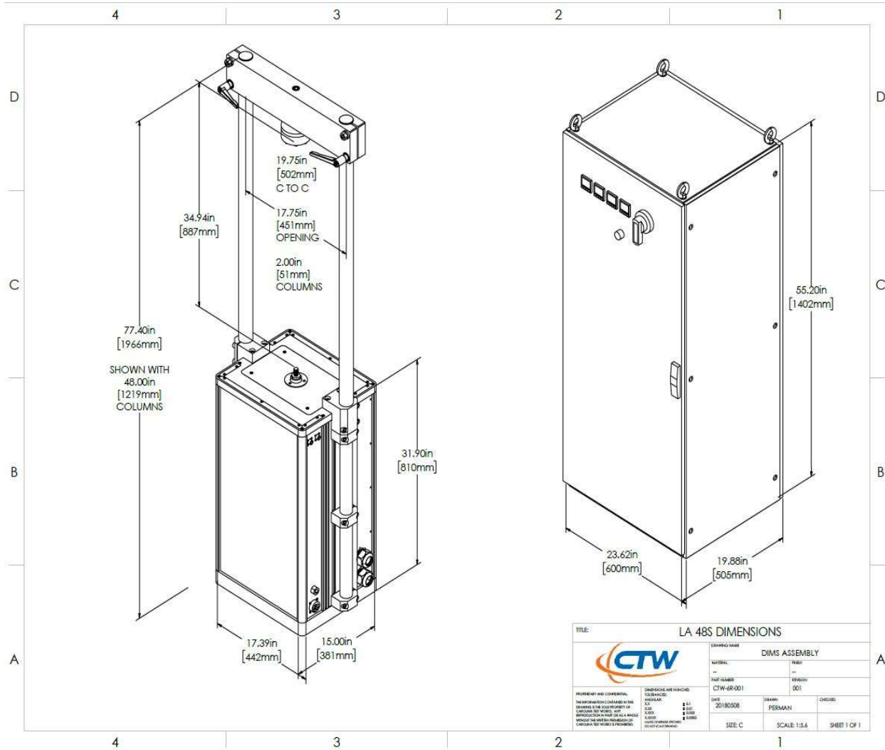
General Dimensional Outline of LA28
